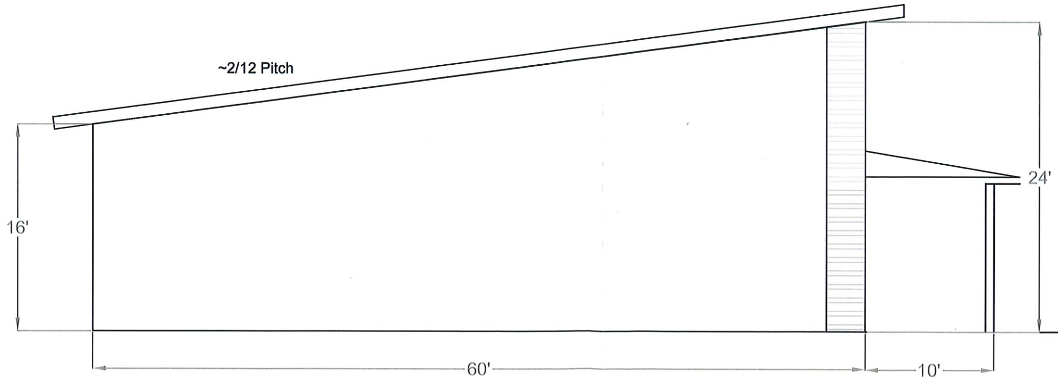
1 ELEVATION EAST VIEW A4 NTS
